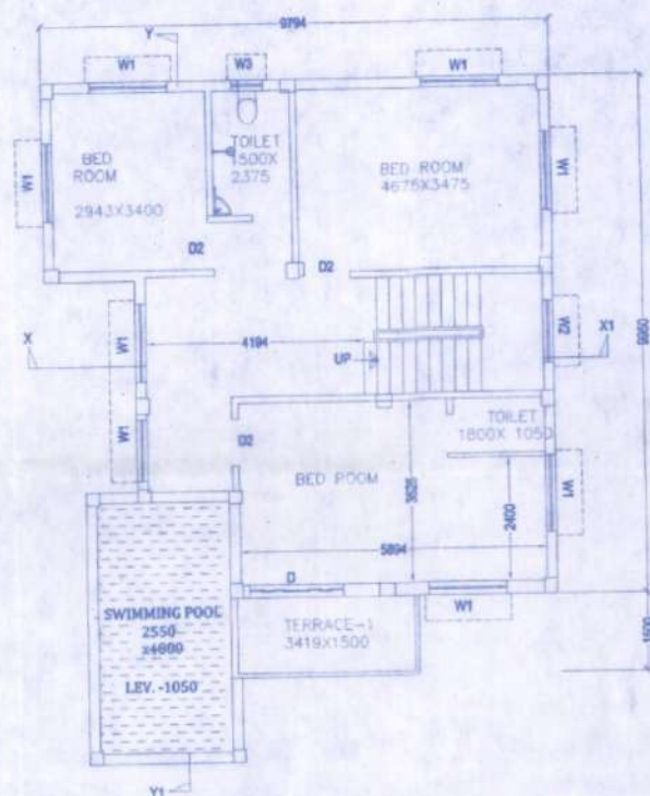
FIRST FLOOR PLAN (BUNGLOW NO.: - NO.: - 81,90,103)
