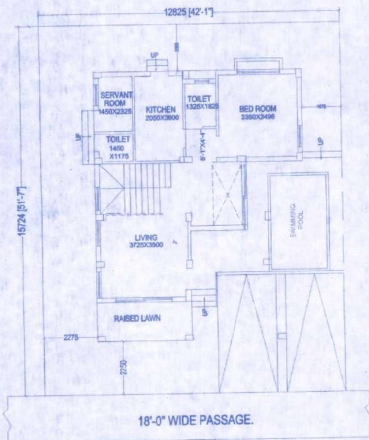
GROUND FLOOR PLAN (BUNGLOW NO-80,102,91)
