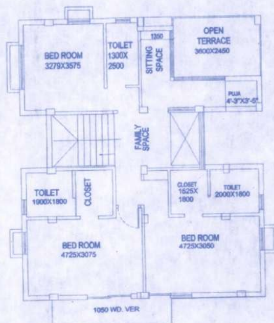
1ST FLOOR PLAN (BUNGLOW NO-80,102,91)
